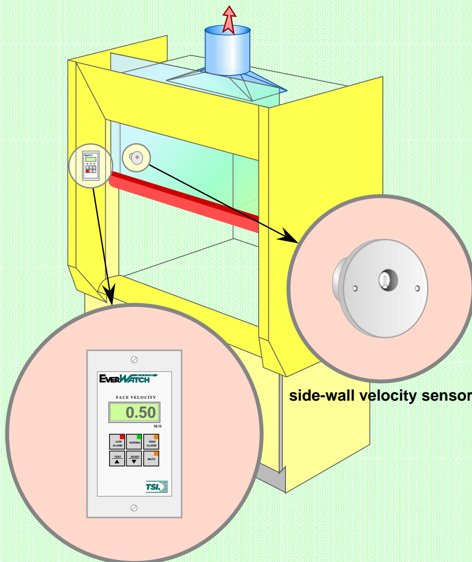
8610 EverWatch monitor/alarm
